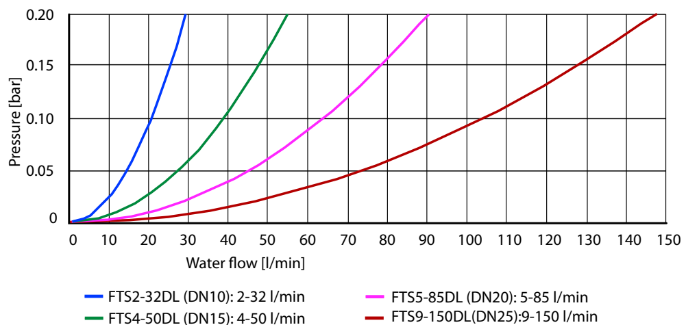
Pressure loss as a function of flow
